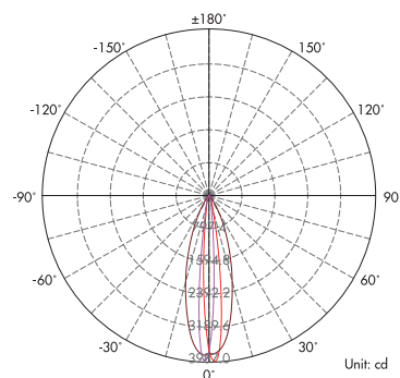
Light Distribution Curve (3000K, 10x30°)
