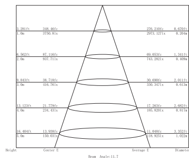
Lux distance Curve (3000K, 10x30°)
