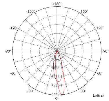
Light Distribution Curve (3000K, 15°40°)
