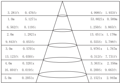
Lux distance Curve (3000K, 30°)
