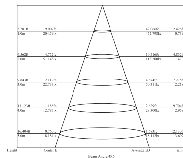
Illumination Picture ( Assymetrical 30° tilt +120° pan beam)
