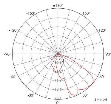
Light Distribution Curve (3000K, 30°x60°)
