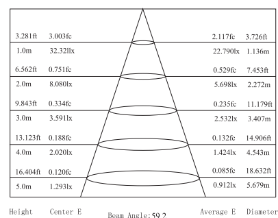
Lux distance Curve (3000K, 30°x60°)
