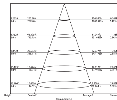
Lux distance Curve (3000K,7W,10x30°)
