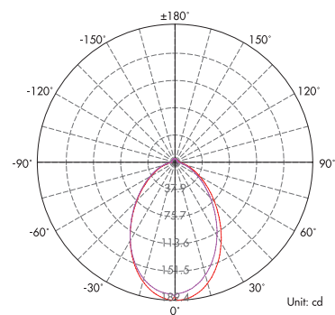
Light Distribution Curve (3000K, 1x120°)
