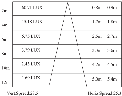
Lux distance Curve (RGBW5500K, 23°)
