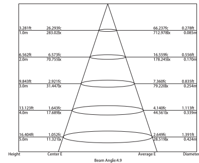
Lux distance Curve (3000K, 300° * 5°)
