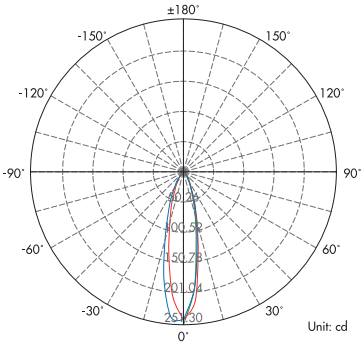
Light Distribution Curve (3000K, 2x80°)
