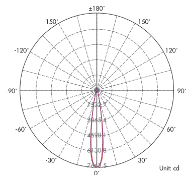
Lux distance Curve (3000K, 10° COB lens )
