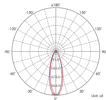
Light Distribution Curve (RGB+CW, 43°)
