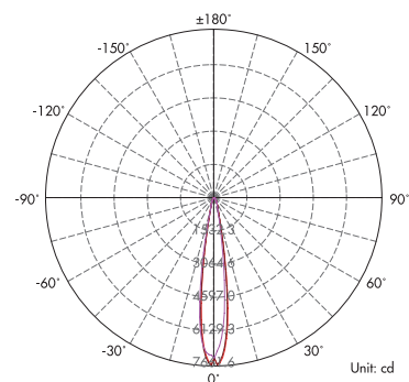
Light Distribution Curve (3000K, 36 °)
