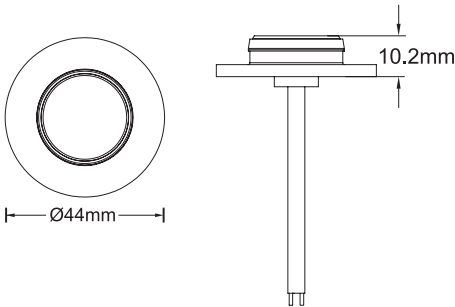
Installation drawing for the lamp body
