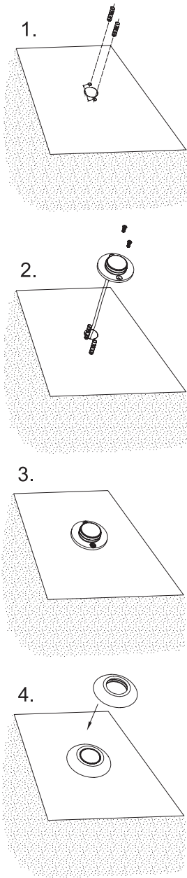
Installation drawing for the lamp body
