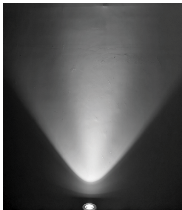
Illumination Picture ( 36°)
