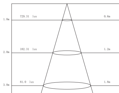
Lux distance Curve (3000K,36°)
