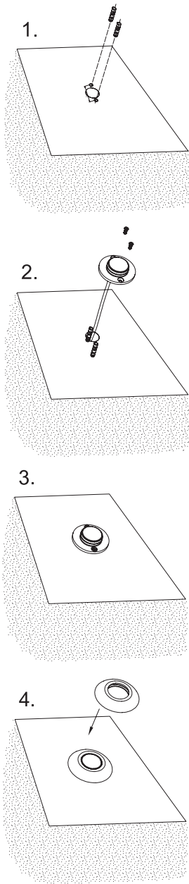
Installation Drawing (It's compatible with the six kinds of cover in the before two pages!)
