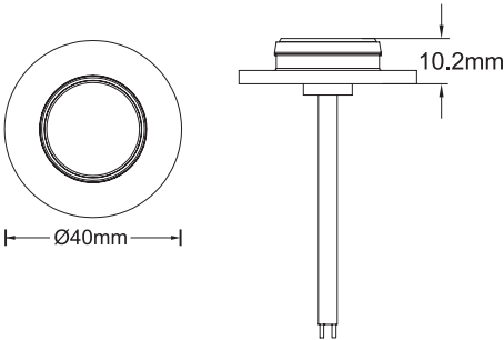
Installation Drawing (It's compatible with the six kinds of cover in the before two pages!)
