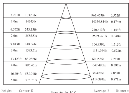
Lux distance Curve (3000K,20°)
