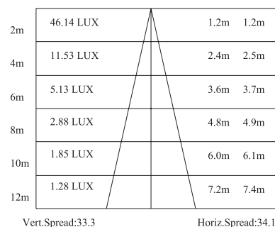
Lux distance Curve (RGBW5500K, 1x30°)
