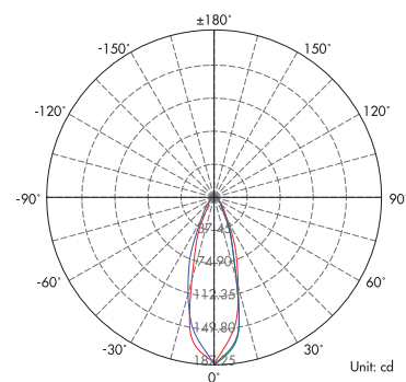
Light Distribution Curve (RGBW5500K, 1x30°)
