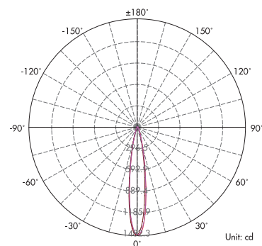
Light Distribution Curve (3000K, 1x15°)
