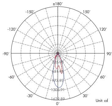
Light Distribution Curve (3000K, 1x38°)
