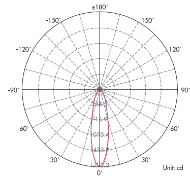
Light Distribution Curve (3000K, 1x40°)
