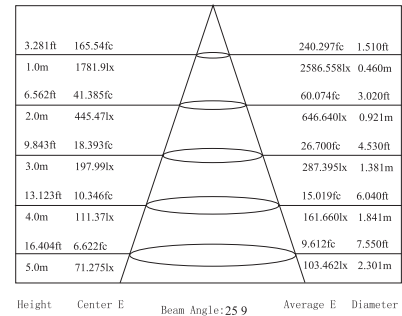
Lux distance Curve (3000K, 1x40°)
