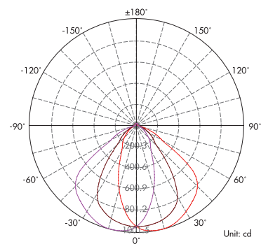
Light Distribution Curve (3000K, 15°+60°)
