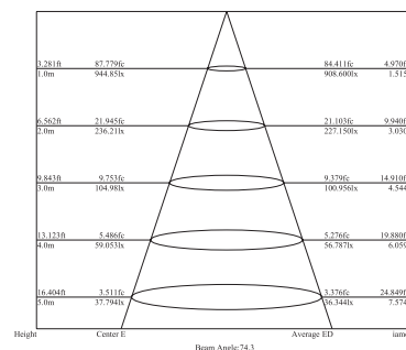
Lux distance Curve (3000K, 15°+60°)
