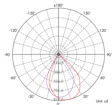
Light Distribution Curve (3000K, 15x70°)
