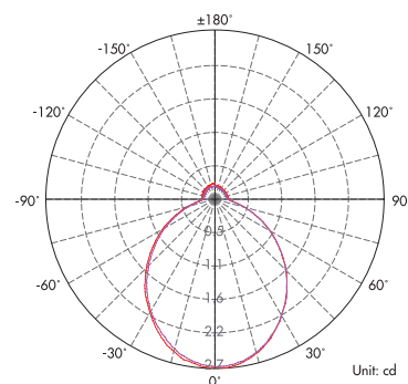
Light Distribution Curve (3000K,360°)
