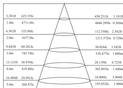
Lux distance Curve (3000K,10°)
