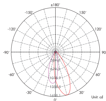
Light Distribution Curve (3000K, 10°+30°)
