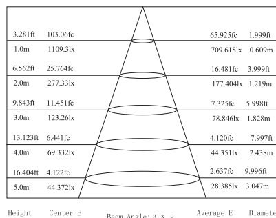
Lux distance Curve (3000K, 10°+30°)
