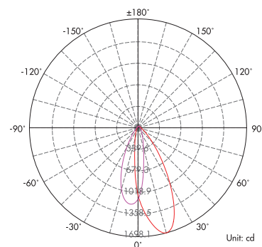
Light Distribution Curve (3000K, 15°+30°)
