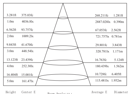
Lux distance Curve (3000K, 17°)
