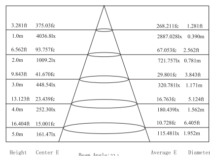
Lux distance Curve (3000K,17°)
