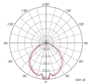
Light Distribution Curve (3000K, 100°)
